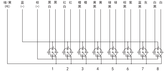
S010-M12D-8C S011-M12D-8C
