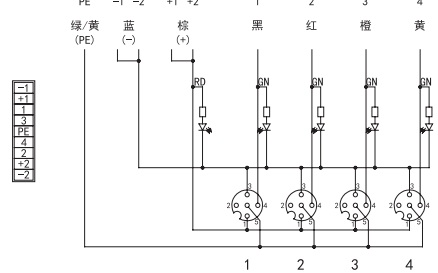
S012-M12-8
