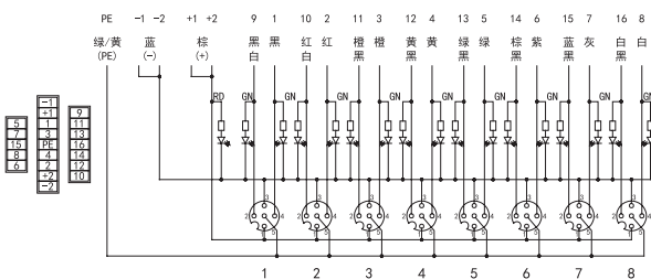
S012-M12D-8P
