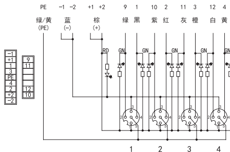
S012-M12D-4
