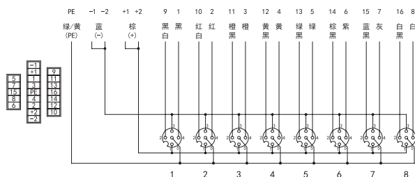
S012-M12D-8C
