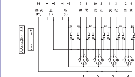
S012-M12D-4P
