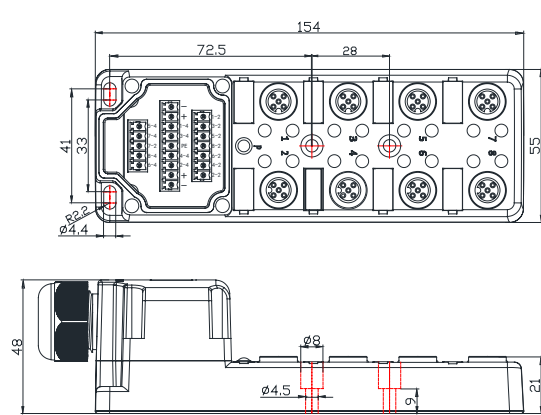
S012-M12-8/8P/8C S012-M12D-8/8P/8C
