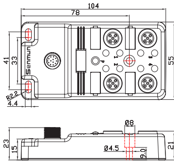
S011-M12-4/4P/4C S011-M12D-4/4P/4C
