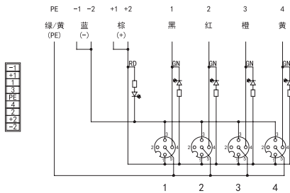
S012-M12-4
