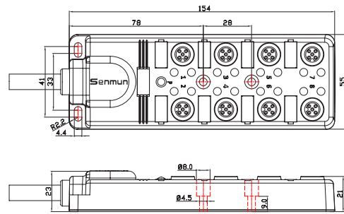
S010-M12-8/8P/8C S010-M12D-8/8P/8C
