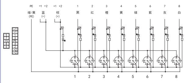
S012-M12-8
