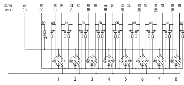
S010-M12D-8 S011-M12D-8
