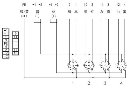
S012-M12D-4C
