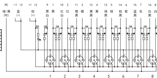
S012-M12D-8C
